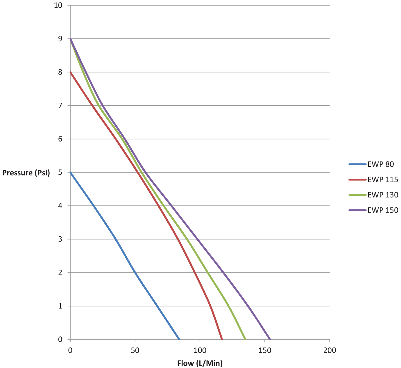
EWP ® Pressure Vs Flow
